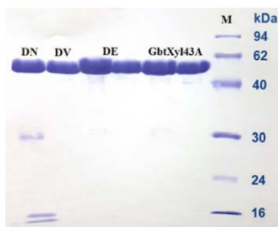
Fig. 2. SDS-PAGE purification profile of \beta -D-xylosidase GbtXyl43A and D121N (DN), D121V (DV) and D121E (DE) mutants, stained with Coomassie Blue; M = protein marker
