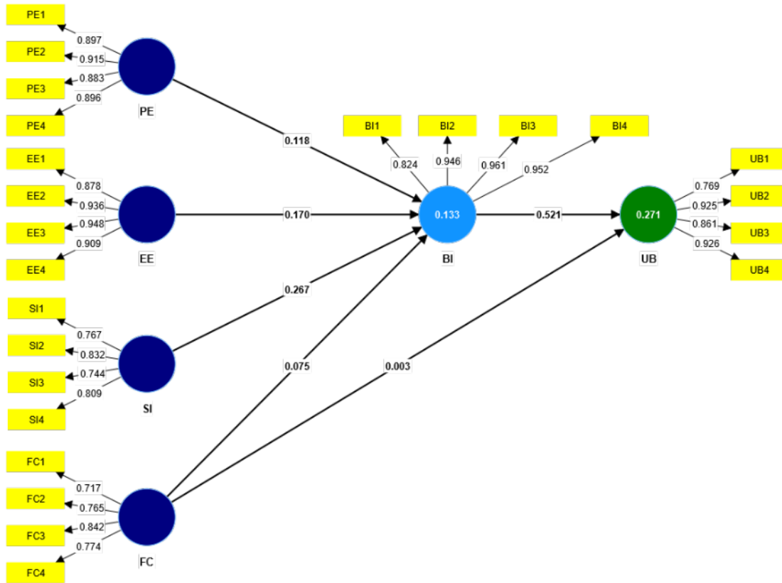
Figure 1. Estimation Results
