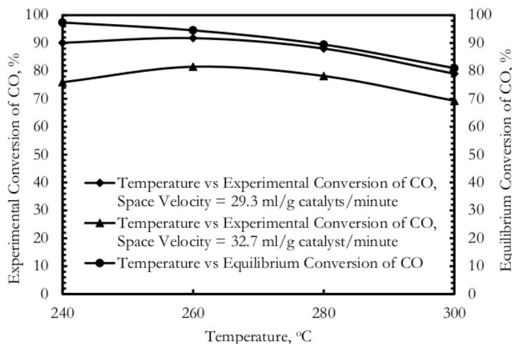
Figure 1. Relationship between temperature on Experimental CO Conversion and Equilibrium CO Conversion for both Space Velocity and CO/H 2 =1/2 mole ratio
