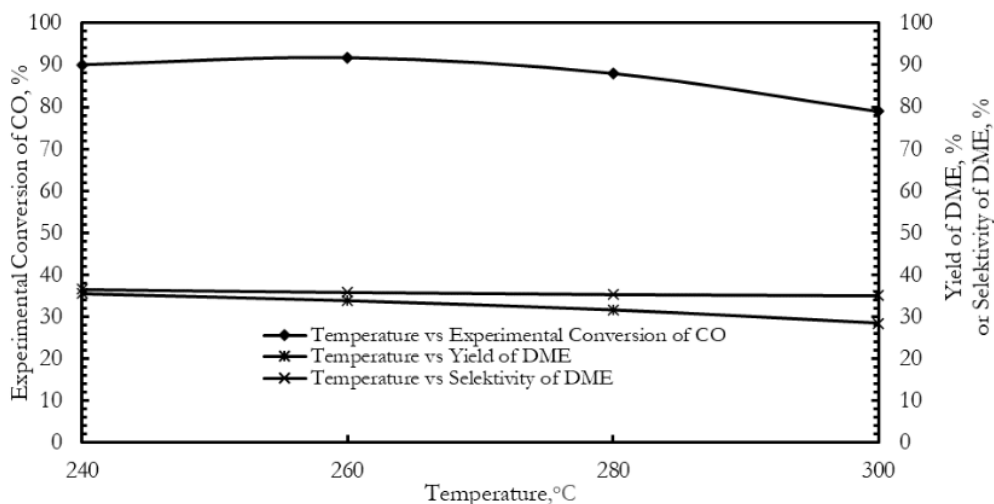
Figure 2. Relationship between temperature on Yield of DME and Selectivity of DME, CO/H 2 mole ratio=1/2, Space Velocity = 29.3 mL/g catalyst/minute
