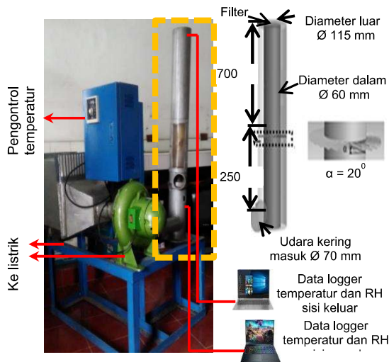
Gambar 5. Alat percobaan pengering swirl fluidized bed
