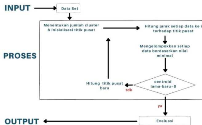
Gambar 2. Diagram Alir Penelitian
