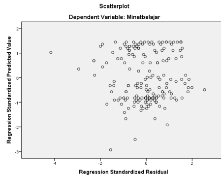
Figure 4. Scatter Plot Linearity Test
