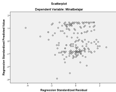
Fig. 4. Scatter Plot Linearity Test
