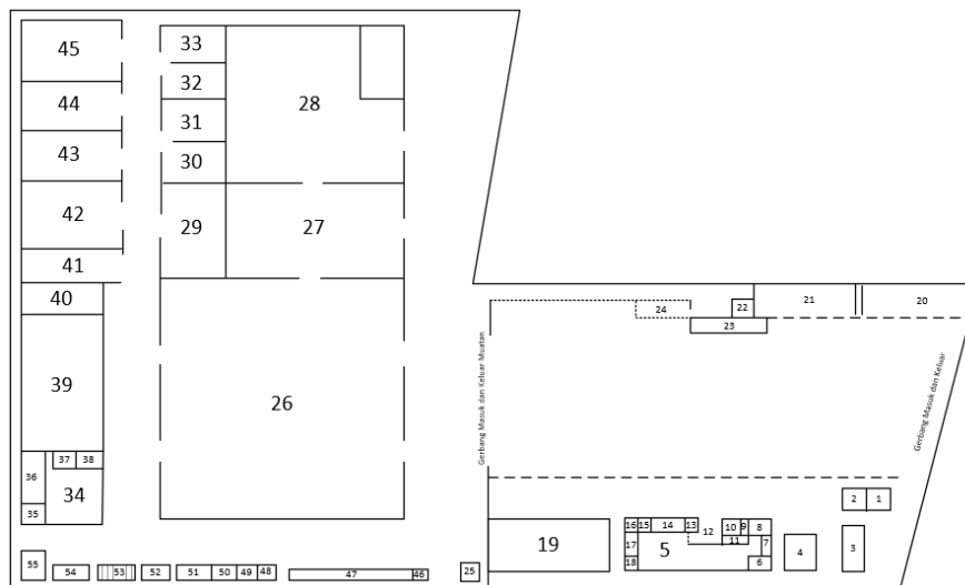
Gambar I.2. Plant Layout Pabrik PT. Menara Jaya Lestari
