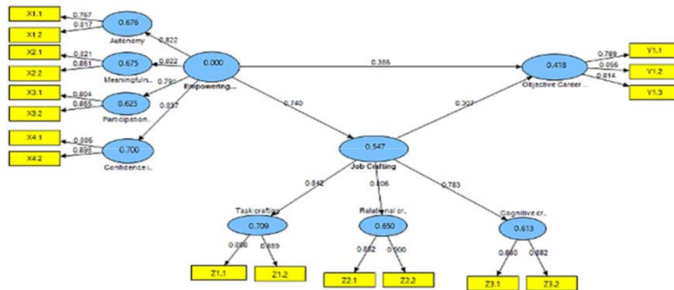
Gambar 1 Uji Outer Model
