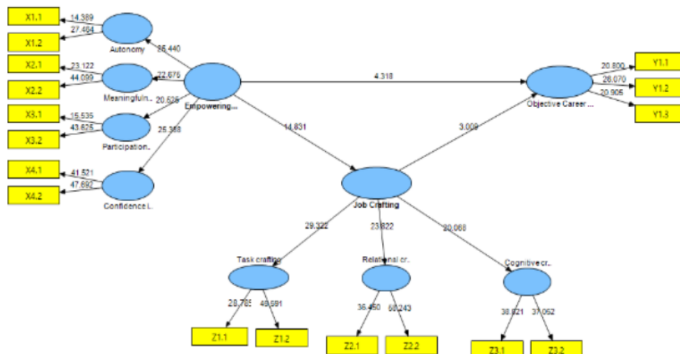
Gambar 3 Uji Inner Model
