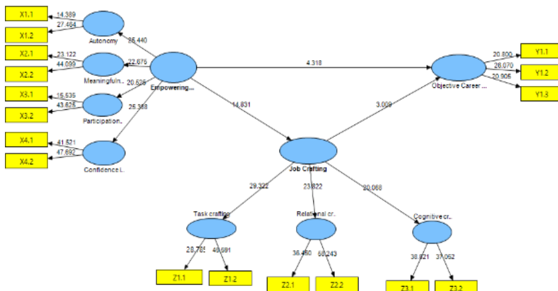
Gambar 3 Uji Inner Model
