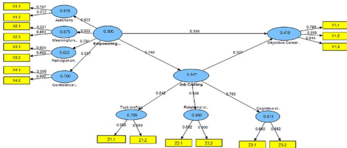
Gambar 1 Uji Outer Model
