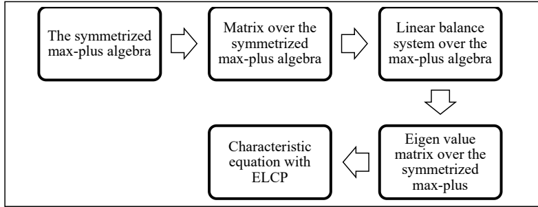
Figure 1. Workflow for the conceptual study of characterization equation of the symmetrized max-plus algebra
