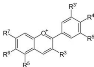
FIGURE 12.1 Chemical structure of anthocyanin.
