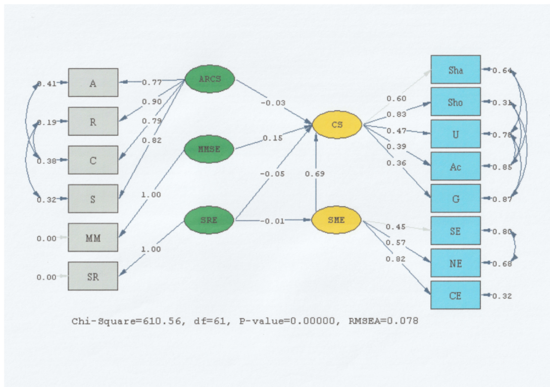
Figure 2 Academic cyberslacking model with standardized loading (N=1485).
