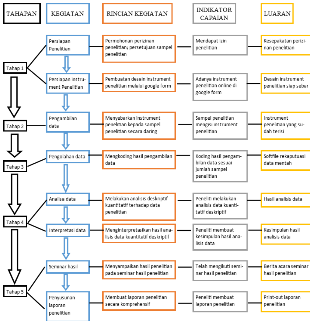
Gambar 2. Alur Penelitian
