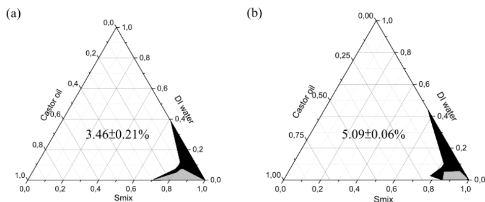
Figure 3. Pseudoternary phase diagram of (a) Tween 20 and (b) Tween 80 with glycerol as the cosurfactant at a weight ratio of 2. The black-colored area refers to the clear, transparent, and one-phase ME region. The grey-colored area refers to the liquid crystal region.
