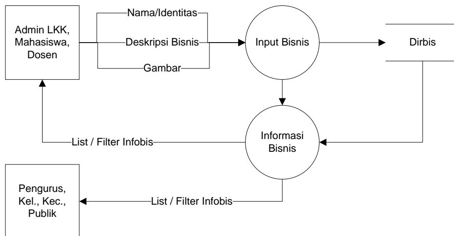
Gambar 8. DFD Context Infobis
