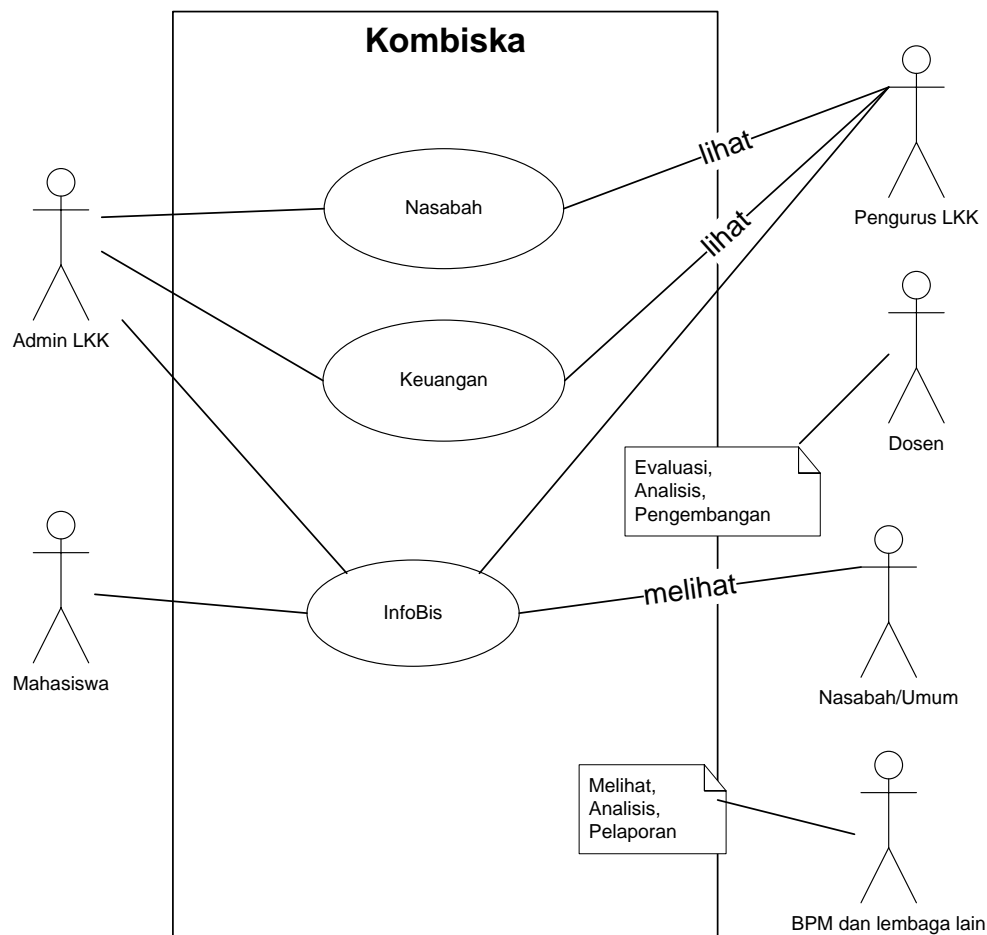
Gambar 3. Use Case Komboka
