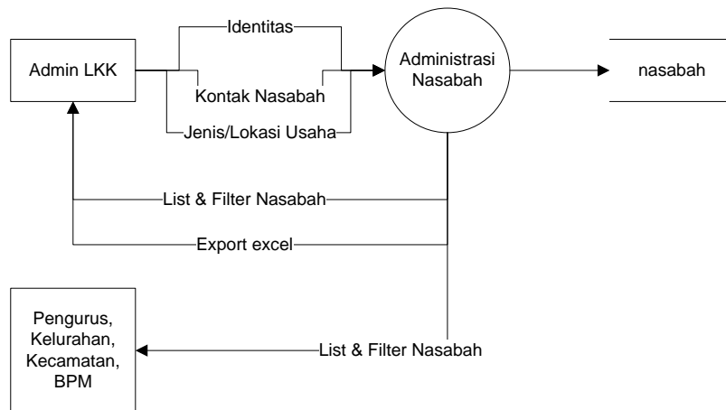
Gambar 7. DFD Context Data Nasabah
