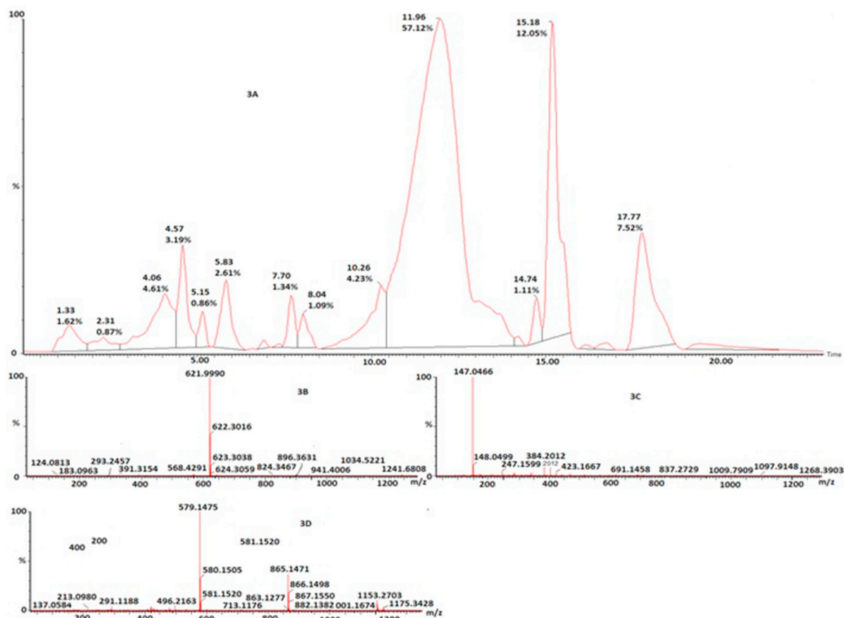
Fig. 3. LCMS of C. burmannii extract (3A) chromatogram peak of UPLC, mass fragments ES positive mode at Rt; (3B) 11.96 min (57.12%) with m/z 621.999; (3C) 7.7 min (1.34%) with m/z 147.0466; (3D) 4.06 min (4.61%) with m/z 579.1475.
