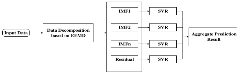
Figure 2. EEMD-SVR Flowcharts
