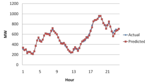
Figure 3. Prediction result on test dataset (1 day observation)
