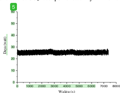
Figure 4.2. CO 2 laser power stability on the line 10R14
