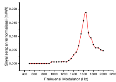
Figure 4.4 Resonance Curve laser lines for ammonia gas
