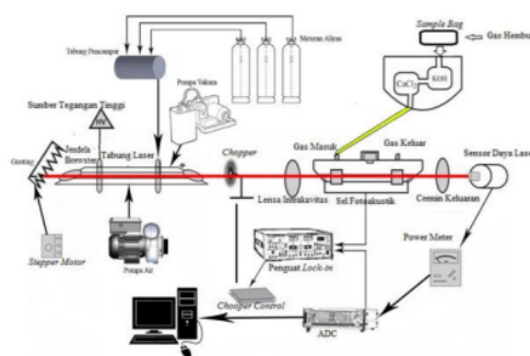
Figure 3.1 Schematic experimental setup in the study using a CO 2 laser photoacoustic spectrometer intrakavitas
