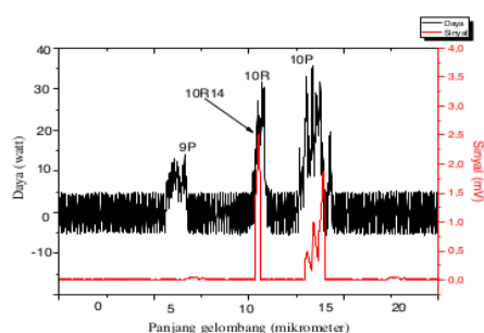
Figure 4.1. Ammonia Absorption Lines
