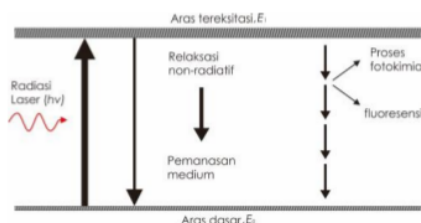
Figure 2.1 Some Type Process Occurred On Ground State Towards Molecular Basis After Radiation Absorbing Laser ( h\nu )
