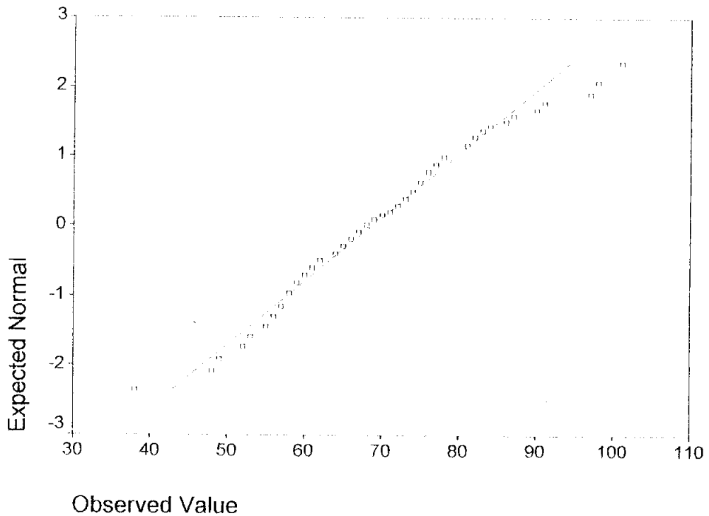
Normal Q-Q Plot of CEMASB
