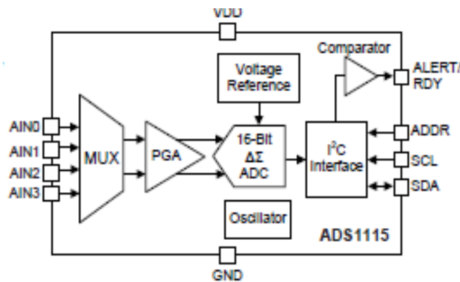
Gambar 5. Diagram blok ADS1115
