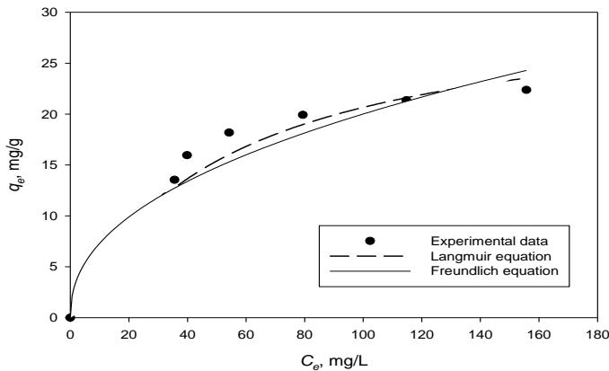
Figure 4 Adsorption isotherm of doripenem on bentonite
