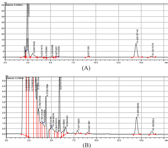
Figure 2. Chromatogram of standard MK (A) and sample (B)
