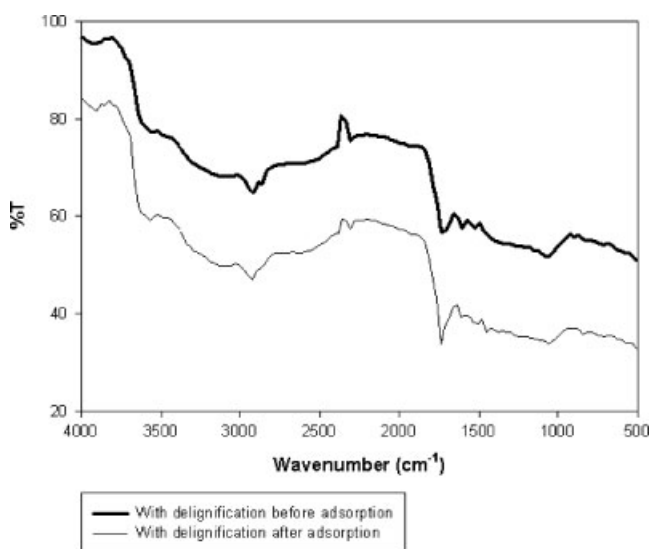
Figure 1. FTIR spectra of neem leaves powder treated with hydrochloric acid at impregnation ratio 1 : 2.5 with delignification process.
