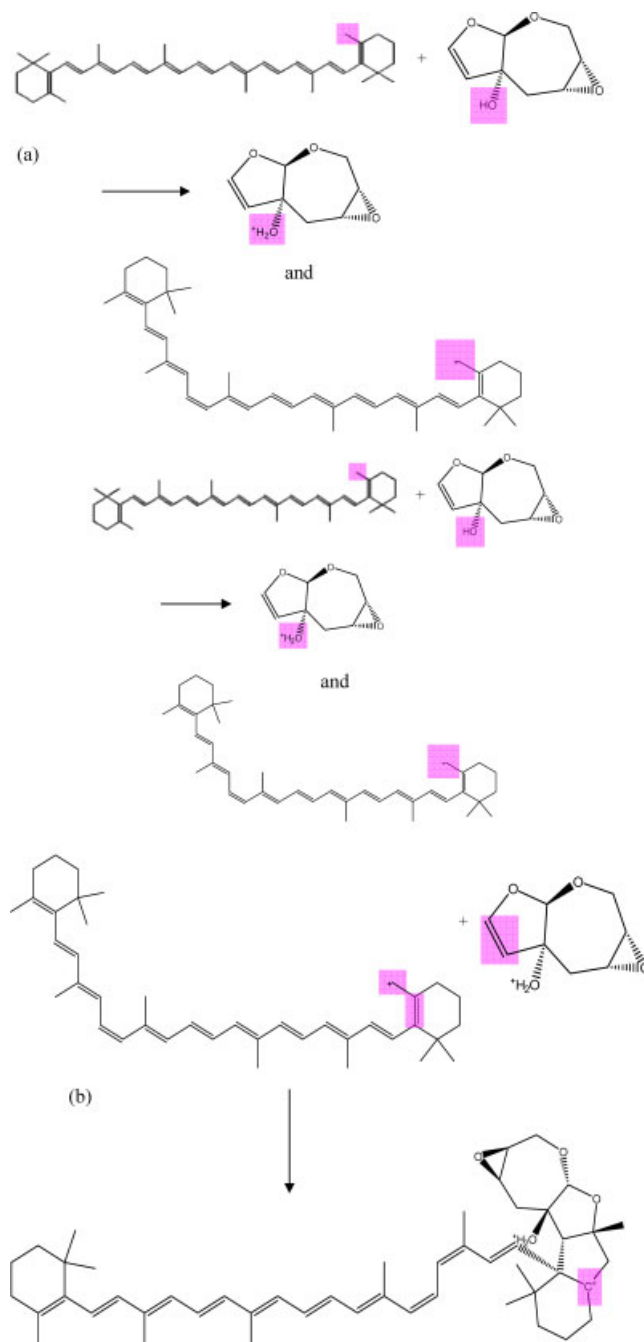
Figure 2. (a) Coordination bonds between hydrogen ion and Lewis site. (b) Adsorption \beta -carotene on active functional group on neem leaves surface. This figure is available in colour online at www.apjChemEng.com .
