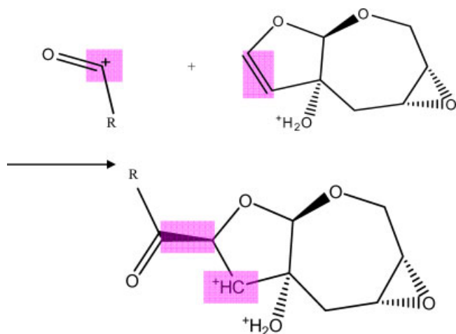
Figure 3. Adsorption secondary oxidation products on active functional group on neem leaves surface. This figure is available in colour online at www.apjChemEng.com .
