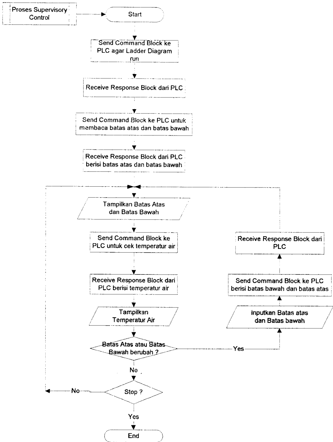
GAMBAR L-3 GAMBAR DIAGRAM ALUR MENU APLIKASI (SUPERVISORY CONTROL) KOMPUTER-PLC
