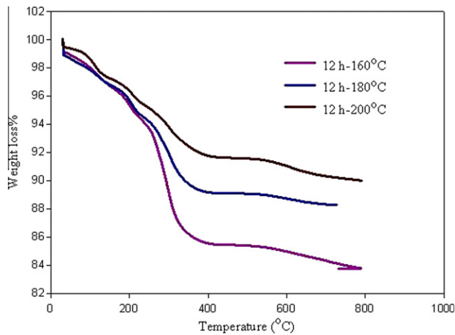
Fig. 7. TGA results for the weight loss as a function of temperature for \text{MnFe}_2\text{O}_4 nanoparticles with \text{PEG}_{300} in different temperature.
