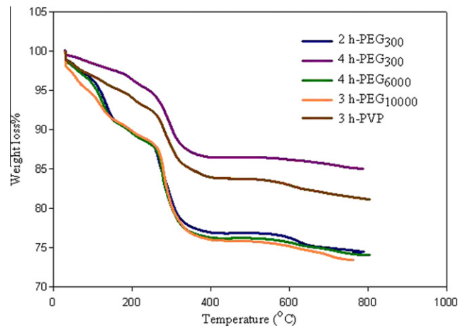
Fig. 8. The weight loss as a function of temperature (TGA) for \text{MnFe}_2\text{O}_4 nanoparticles with different surfactants (200 °C).
