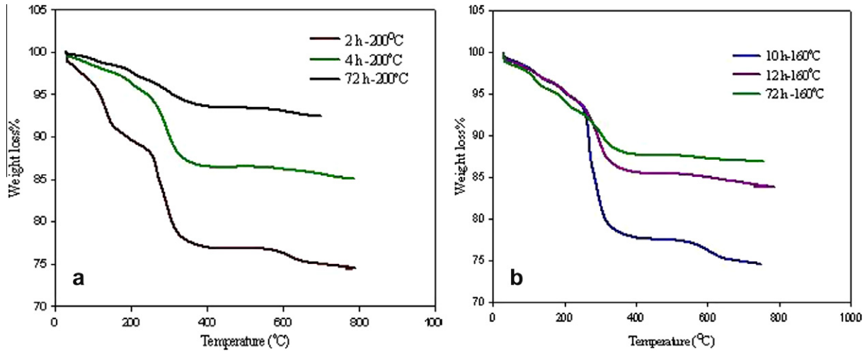
Fig. 6. The weight loss as a function of temperature (TGA) for \text{MnFe}_2\text{O}_4 nanoparticles with \text{PEG}_{300} for different time (a) 200 °C, (b) 160 °C.
