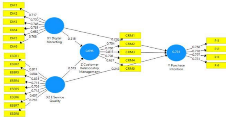
Gambar 2 Outer Model
