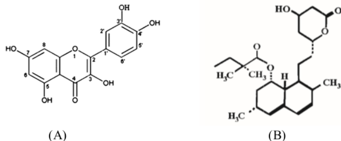
Gambar 4. Struktur flavonoid (A) dan struktur simvastatin (B) (Istvan and Deisenhofer, 2001; Stancu and Sima, 2001).
