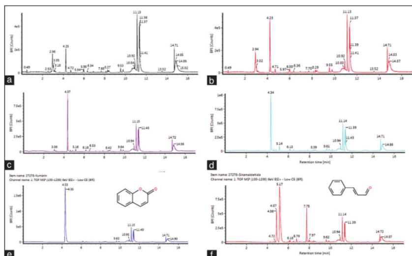
Figure 4: The LC results of the PI, NI infusions, PS, NS Soxhlet extraction, coumarin, and cinnamaldehyde (a) PI, (b) NI, (c) SP, (d) NP, (e) coumarin, and (f) cinnamaldehyde
