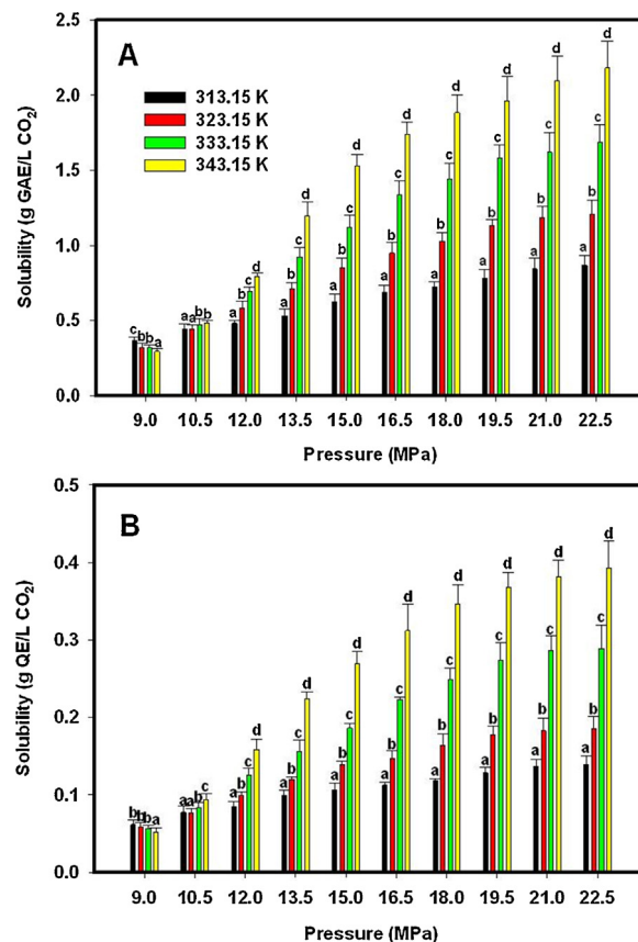
Fig. 3. Solubilities of total polyphenols (A) and total flavonoids (B) in SC-CO 2 at various pressures and temperatures (error bars represent standard deviation), values not sharing same letters are significantly different ( p < 0.05 ) based on one-way analysis of variance and Duncan's multiple range tests.
