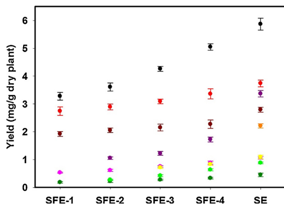
Fig. 2. Extraction yields of several phenolic compounds (● quercetin; ● gallic acid; ● p -coumaric acid; ● rutin; ● luteolin; ● kaempferol; ● ferulic acid; ● (+)-catechin; and ● caffeic acid) obtained from soxhlet extraction and SC-CO 2 extraction at a pressure of 22.5 MPa and various temperatures (SFE-1/313.15 K; SFE-2/323.15 K; SFE-3/333.15 K; and SFE-4/343.15 K).
