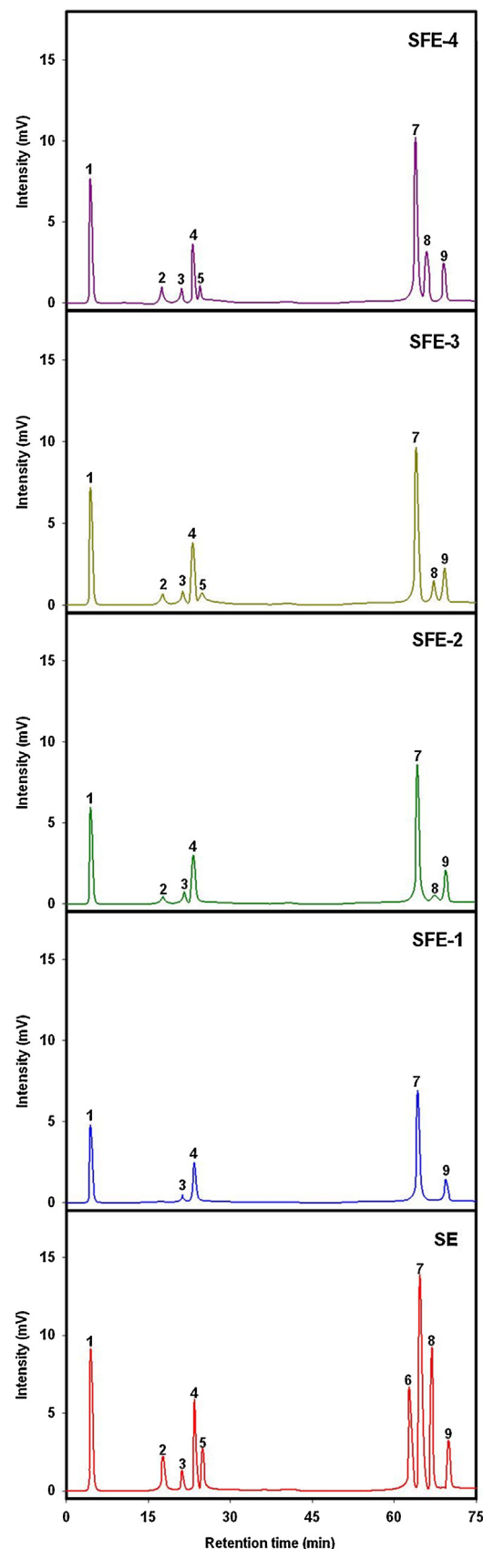
Fig. 1. HPLC chromatograms of antioxidant extracts obtained from soxhlet extraction and SC-CO 2 extraction. The identified compounds are designated by numbers as follows: gallic acid (1); (+)-catechin (2); caffeic acid (3); p -coumaric acid (4); ferulic acid (5); rutin (6); quercetin (7); luteolin (8) and kaempferol (9).
