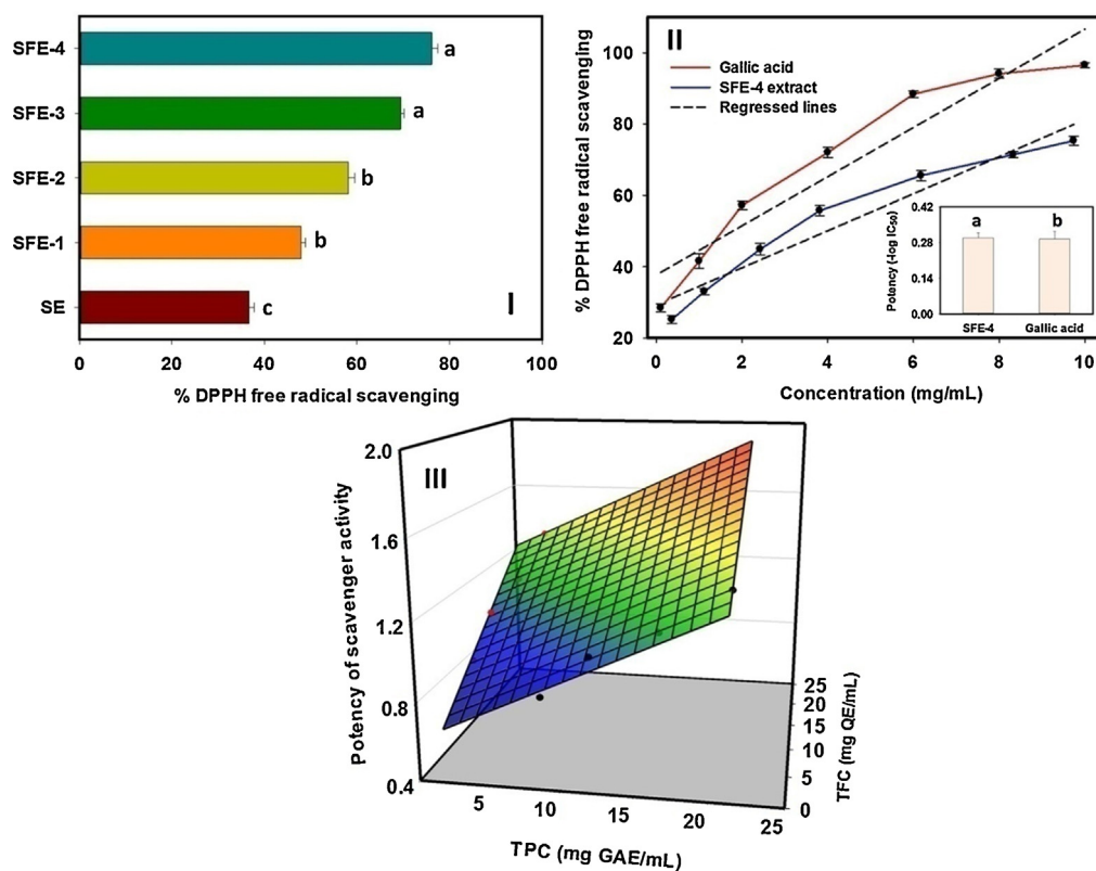
Fig. 5. Scavenging percentage of various antioxidant extracts, different letters indicate significant differences between means (I), DPPH-scavenging activity between SFE-4 extract and gallic acid (inset is the potency values ( P ), determined as -\log (IC_{50}) ) (II), and 3D-linear correlation between scavenging potency and bioactive contents (● TPC and ● TFC) of SFE extracts (III).
