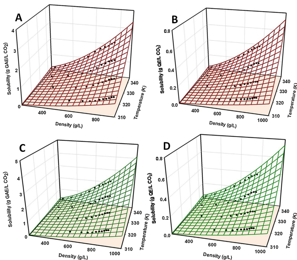
Fig. 4. 3D-fitting of Chrastil (A–B) and Del Valle–Aguilera (C–D) models on the experimental solubilities of polyphenols (g GAE/L CO 2 ) and flavonoids (g QE/L CO 2 ).
