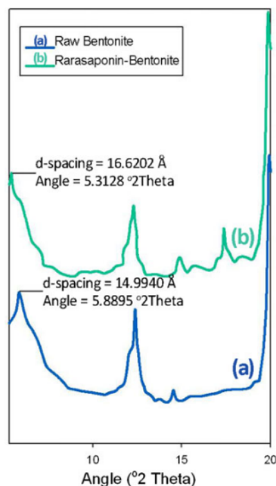
Fig. 3 XRD results of natural bentonite and rarasaponin-bentonite
