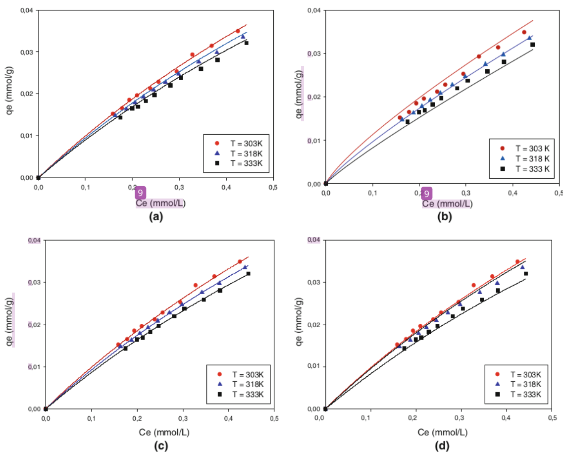
Fig. 4 Adsorption experimental data of Evans blue onto natural bentonite and the model fitted by a Langmuir, b Freundlich, c Sips, and d Toth isotherms
