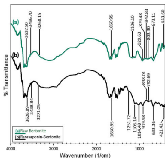
Fig. 2 FTIR spectra of natural bentonite and rarasaponin-bentonite
