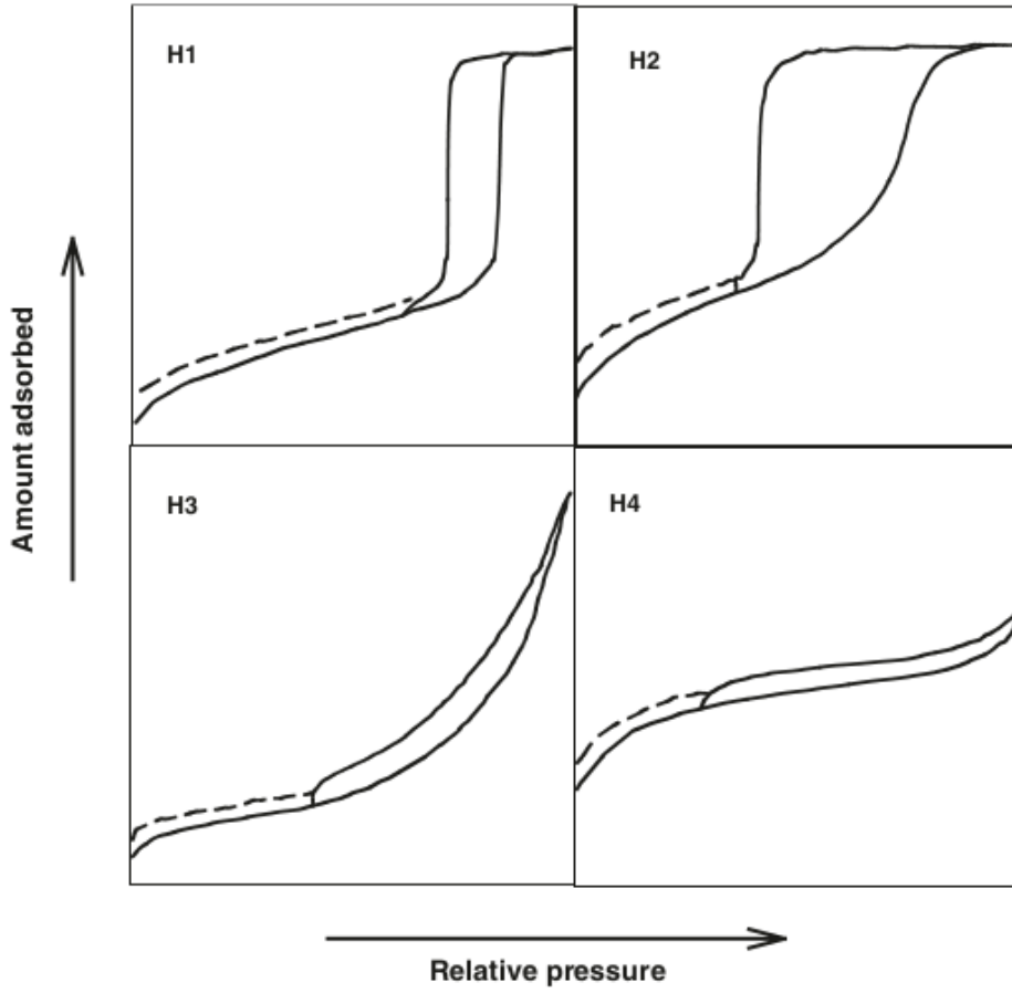
Fig. 5.2 Relation between the hysteresis of sorption isotherm and the pore shape (Alothman 2012)
