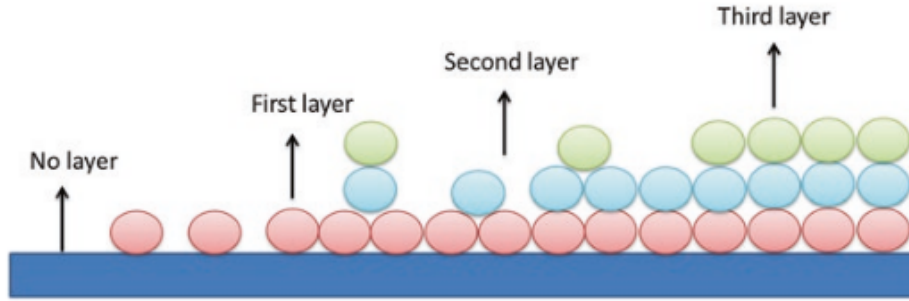
Fig. 4.4 Multiple layering in BET theory (Do 1998)
