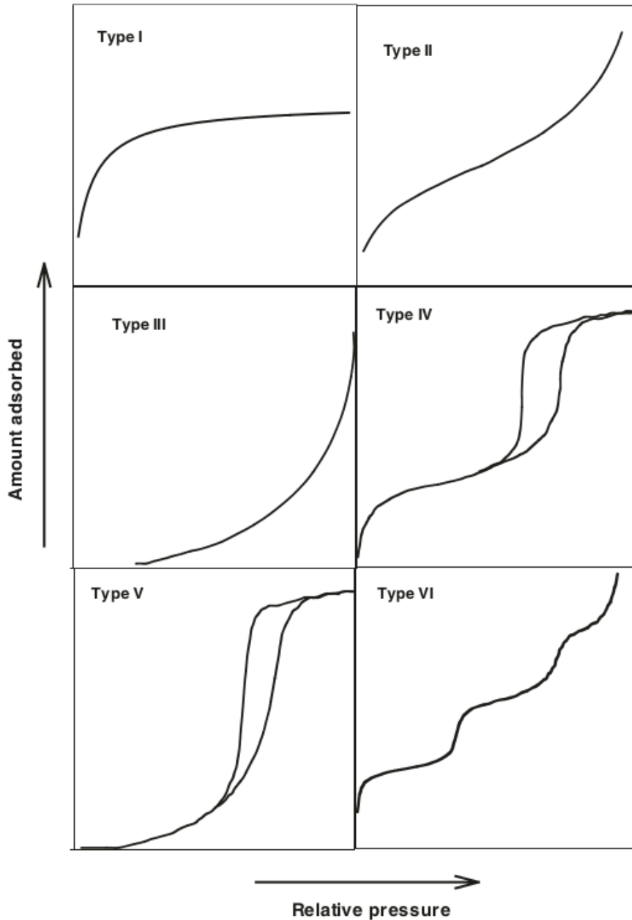
Fig. 5.1 The IUPAC classification of adsorption isotherm (Alothman 2012)
