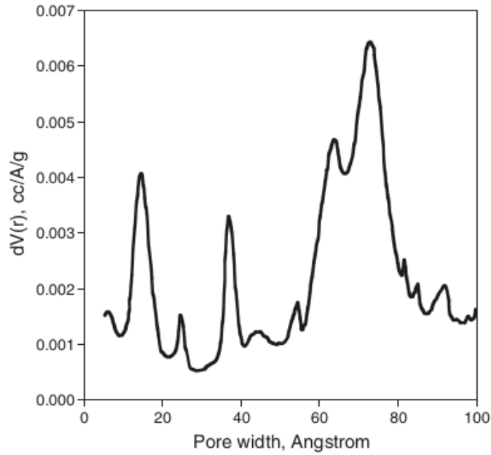
Fig. 5.4 The DFT pore size distribution of bentonite from Pacitan
