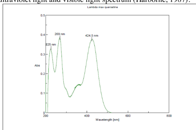
Figure 1. Maximum Wavelength
