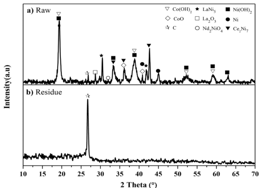
Fig. 3. XRD patterns of a) raw sample powder from spent NiMH batteries and b) residue after aqua regia digestion.
