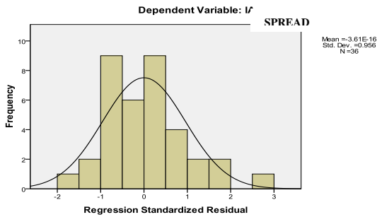
Histogram
