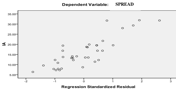
Scatterplot
