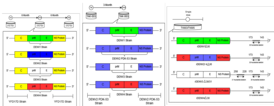
Figure 1. Structure of: (a) CYD -TDV (Dengvaxia); (b) TAK -003; (c) TV003 / TV005
