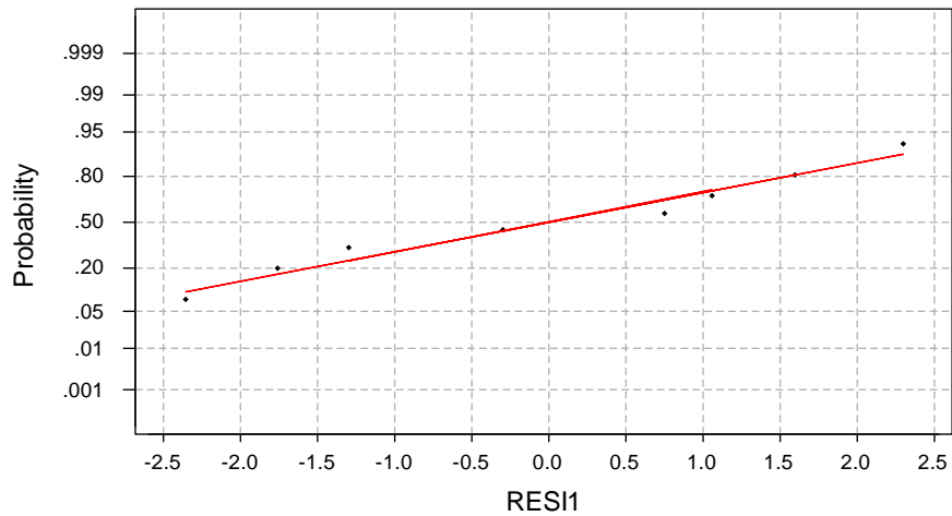
Normal Probability Plot
