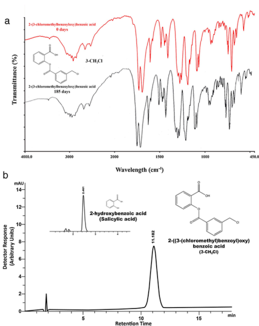
Fig. 5. A fingerprint of the 3-CH 2 Cl compound.
