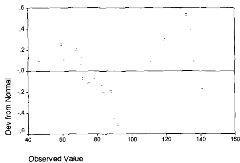
Detrended Normal Q-Q Plot of TOTAL
