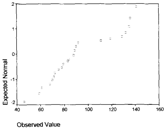
Normal Q-Q Plot of TOTAL
