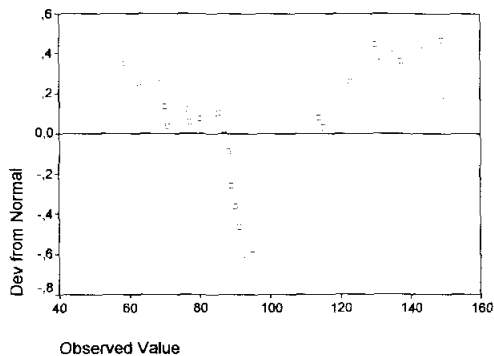
Detrended Normal Q-Q Plot of TOTAL
