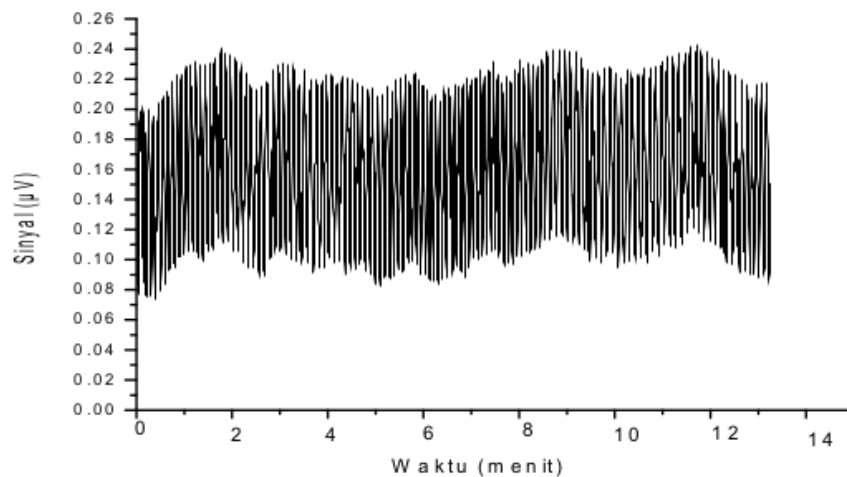
Figure 3.1 CO 2 laser noise
