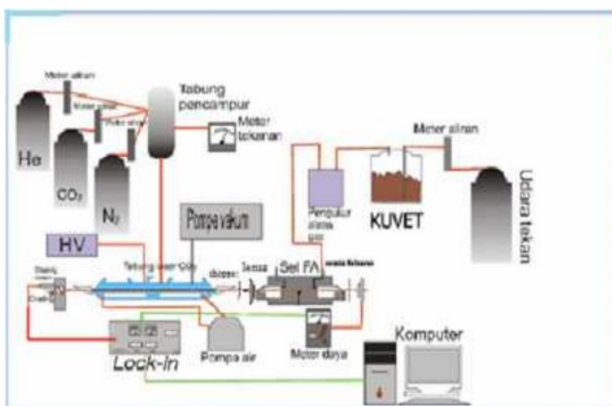
Figure 2.1 Laser CO_2 photoelectric spectroscopy kit
