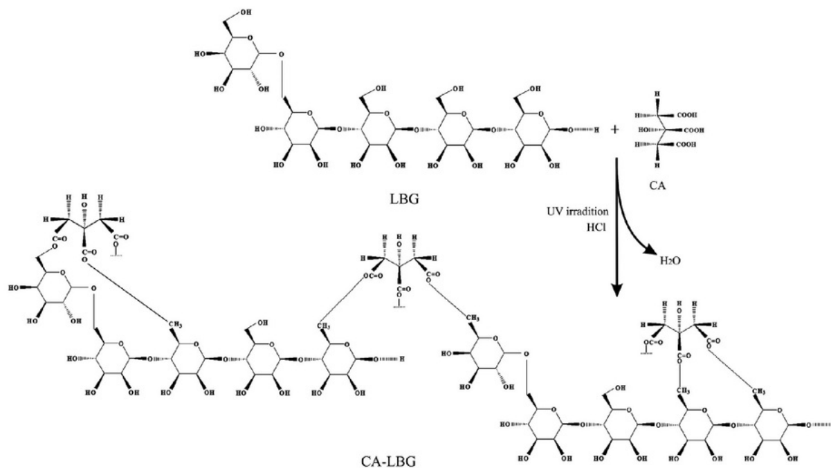
Fig. 1. Proposed mechanism esterification CA with LBG.
