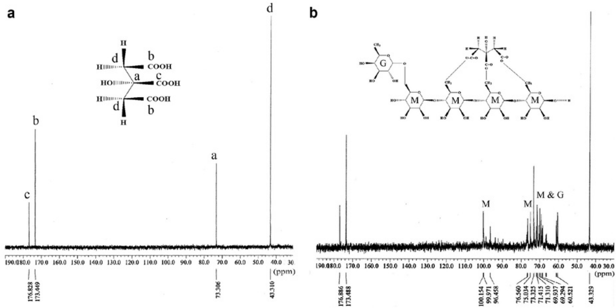
Fig. 3. a. 13 C NMR spectrum of CA. b. 13 C NMR spectrum of CA-LBG representative of various condition (condition 2).
