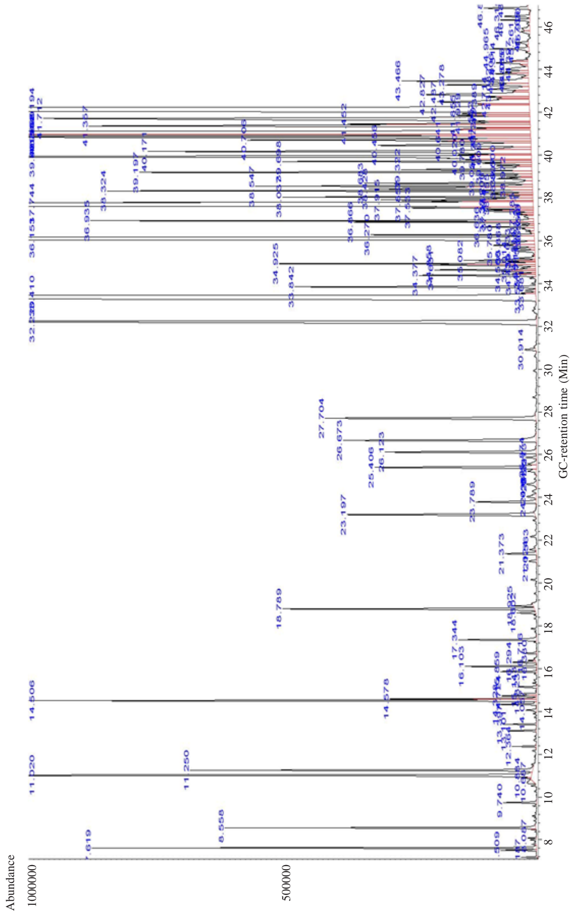
Figure 1. Chromatogram of volatile compounds in Pluche indica Less essential oil.
